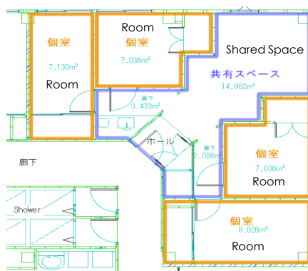
Unit Layout
